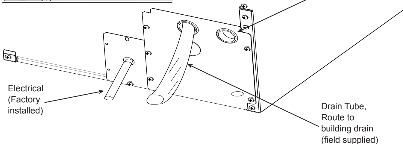
Back View, Drain Pump Model
